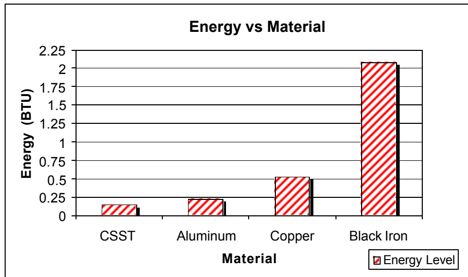
Figure 2: Comparison of heat capacity for 100 mil diameter hole in CSST, Aluminum Copper & Black Iron
